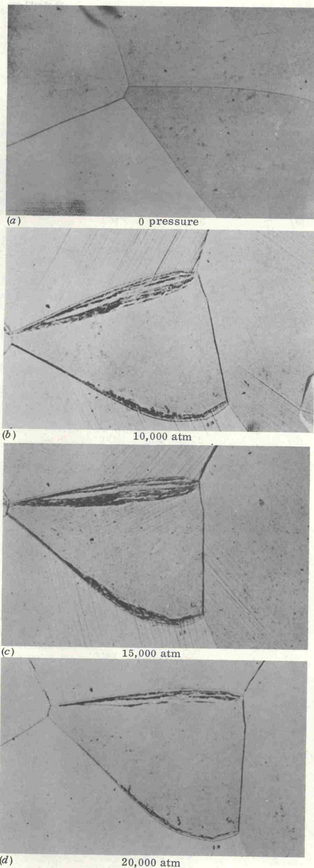
Fig. 3—Localized structural change adjacent to boundaries with slip continuing across original boundaries. X100. Enlarged approximately 9 pct for reproduction.
