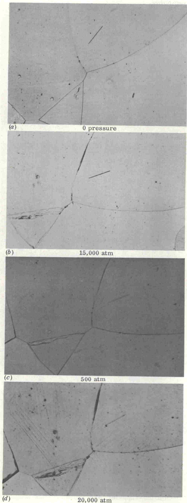
Fig. 2—Typical structural changes along one side of original grain boundary. X100. Enlarged approximately 2 pct for reproduction
